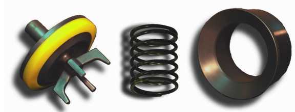
Premium wing guided valve, spring, & full open seat
